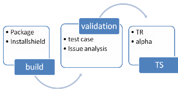
Figure 2: Proposed model
