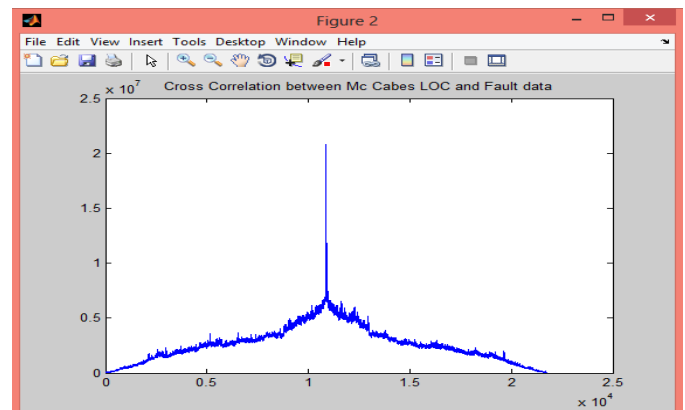
Figure 9: Cross Correlation between Mc Cabes LOC and Fault Data
