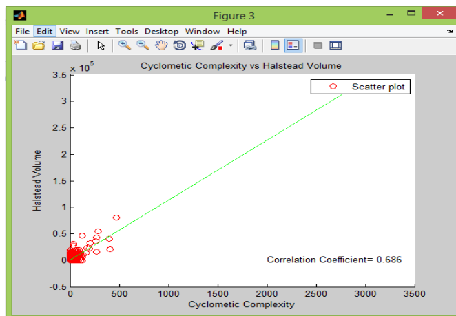
Figure 4: Correlation between Cyclomatic Complexity and Halstead Volume
