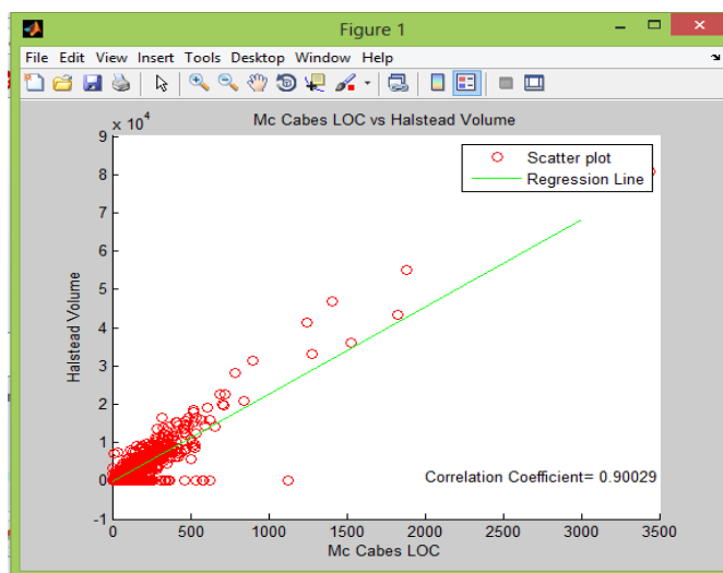
Figure 2: Correlation between Mc Cabes LOC and Halstead Volume
