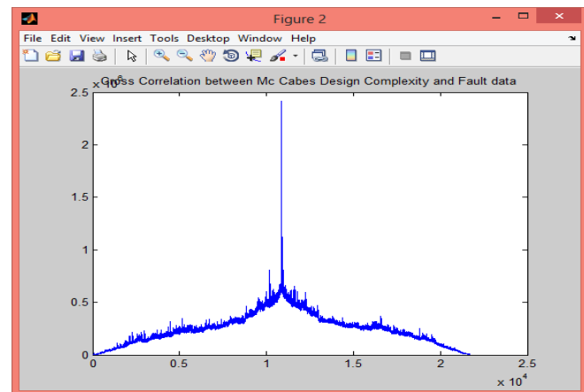
Figure 13: Cross Correlation between Mc Cabes Design Complexity and fault data
