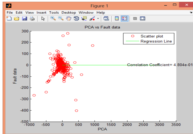
Figure 19: Correlation between PCA reduced data and fault data
