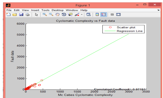
Figure 10: Correlation between Mc CabesCyclomatic Complexity and Fault data
