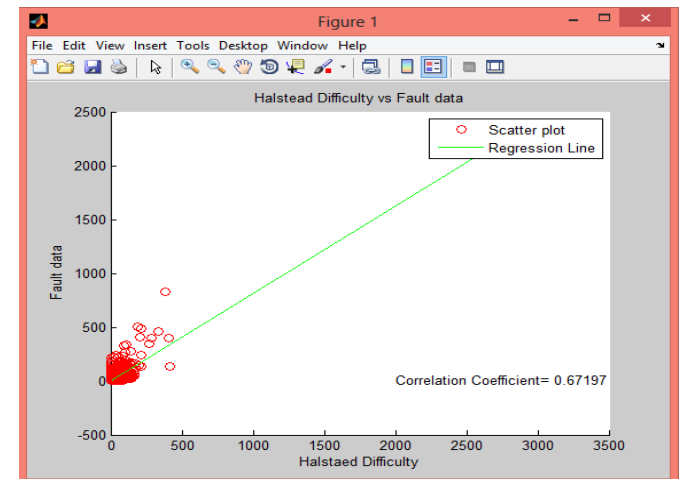
Figure 16: correlation between Halstead Difficulty and fault data
