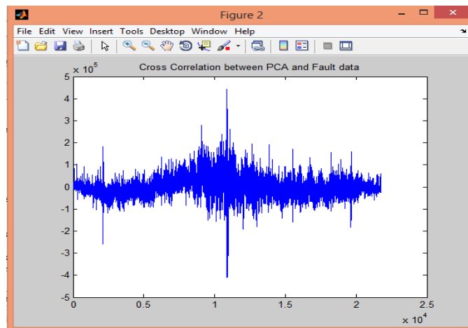
Figure 20: Cross Correlation between PCA reduced data and fault data
