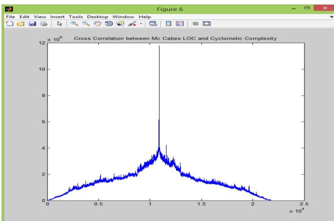
Figure 7: Cross correlation between Mc Cabes LOC and Cyclomatic Complexity
