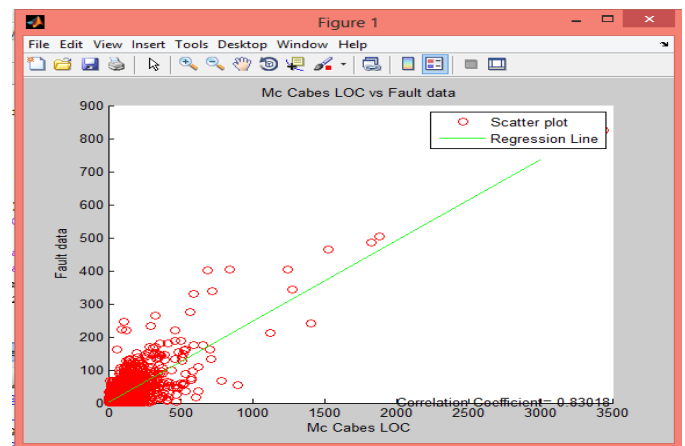
Figure 8: Correlation between Mc Cabes LOC and Fault Data
