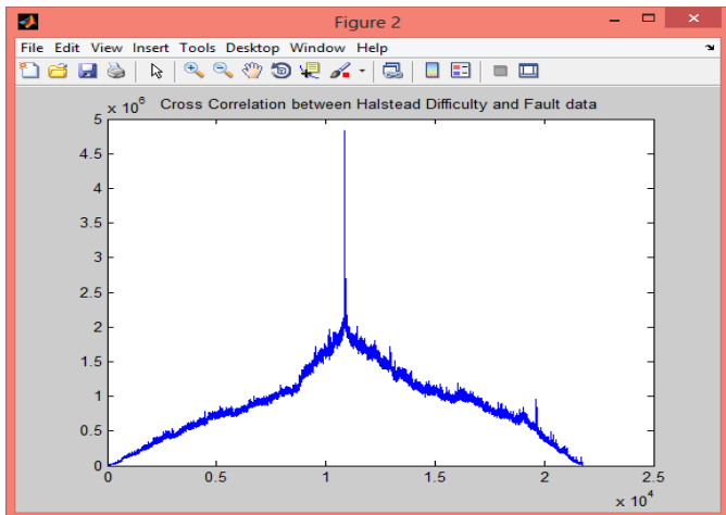
Figure 17: Cross correlation between Halstead Difficulty and fault data
