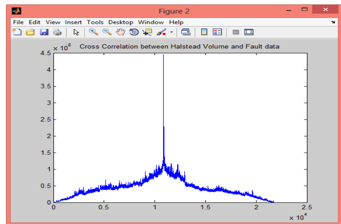
Figure 15: Cross Correlation between Halstead Volume and Fault data
