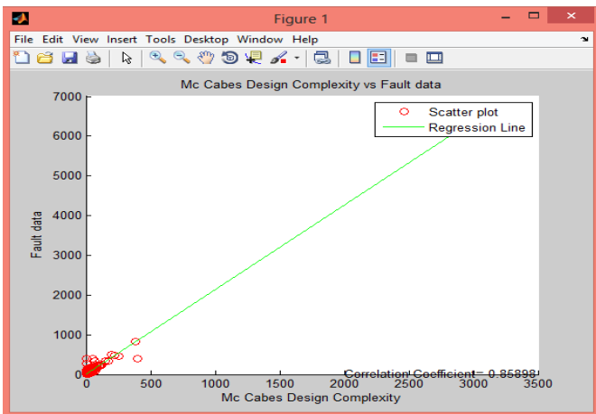
Figure 12: Correlation between Mc Cabes Design Complexity and fault data
