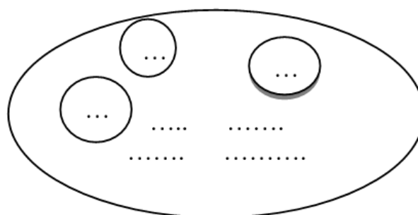
Figure 2: Clustering Nodes
